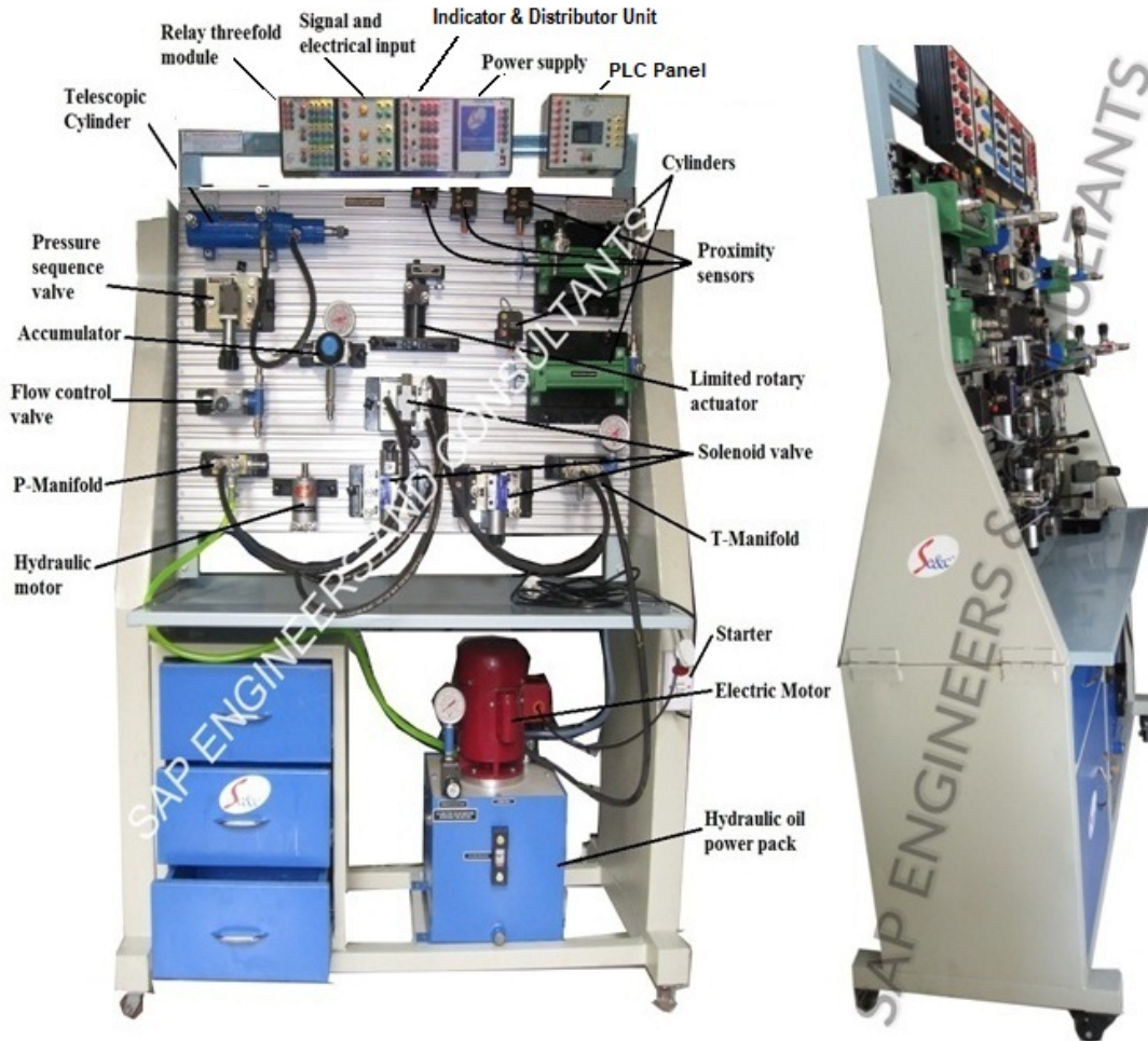
ADVANCED CUSTOMIZED ELECTRO-HYDRAULIC TRAINER (SAP-38 D)
